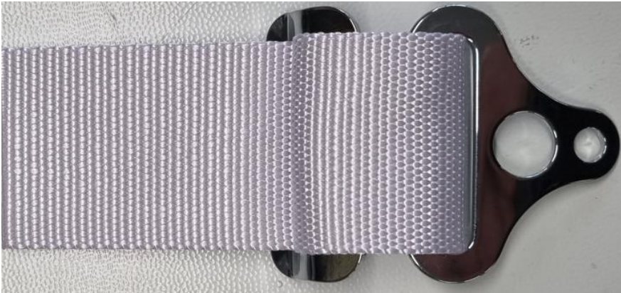
ALTERNATIVE ATTACHMENT PLATE CS051PI00 + Z PLATE CS050PI00 ON PELVIC STRAP
