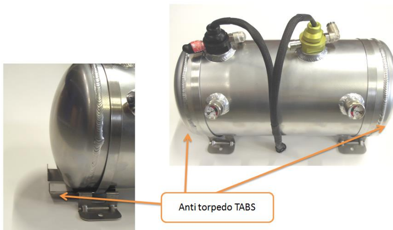
Fig. 5 Anti torpedo tabs
