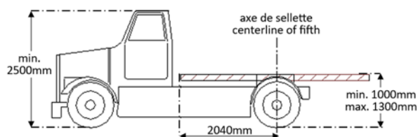
Dessin / Drawing 290-3.17.1
