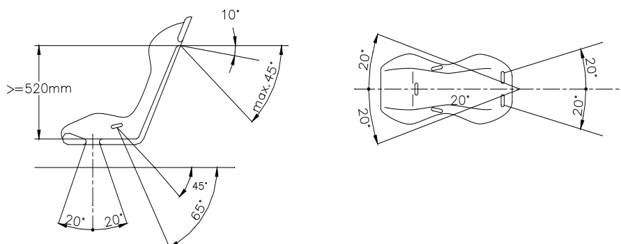
Dessin / Drawing 253-61
