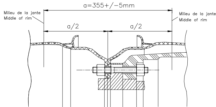
Dessin / Drawing 290-3.14
