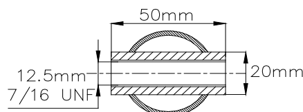
Dessin / Drawing 253-67
