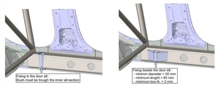
Dessin / Drawing 279E-13
