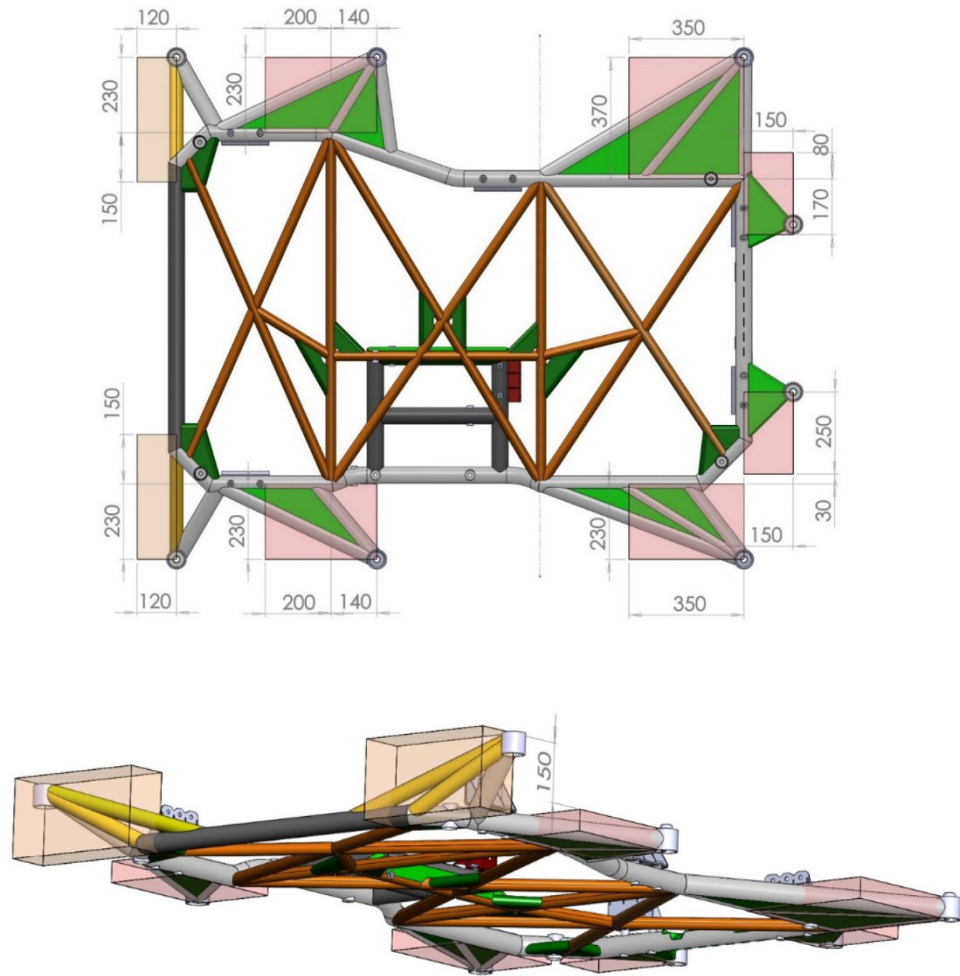
Dessin / Drawing 279E-2
