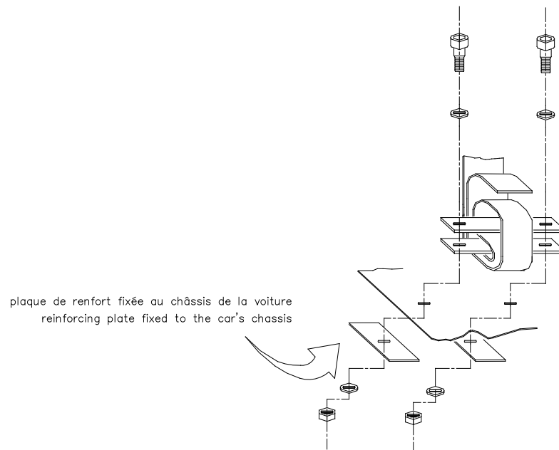
Dessin / Drawing 253-64
