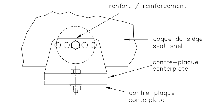
Dessin / Drawing 253-65
