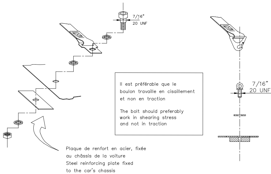
Dessin / Drawing 253-62
