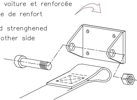
Dessin / Drawing 253-63
