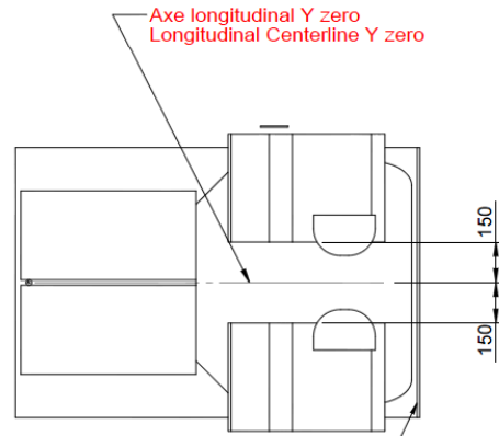
Face Avant Structure de securite Arriere Front Face of Rear Rollover Structure
