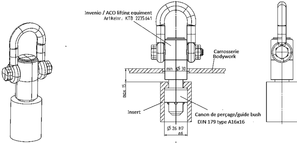
Insert detail
